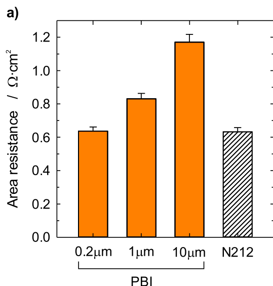
Figure 3. (a) Area specific resistance measured in situ after conditioning of the cell for 4 h in \text{V}^{+3.5} electrolyte (state of charge of \sim 50\% ). (b) Charge/discharge curves recorded at room temperature and a current density of 150 \text{ mA}\cdot\text{cm}^{-2} . Electrodes: Toyobo AAF304ZS (compression: 28%). 40 ml of vanadium electrolyte on each side (nominal capacity: 1.72 Ah), flow rate: 50 \text{ ml}\cdot\text{min}^{-1} .
